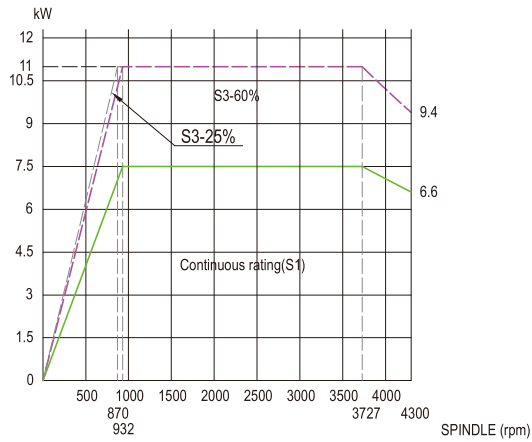
Horsepower Chart
