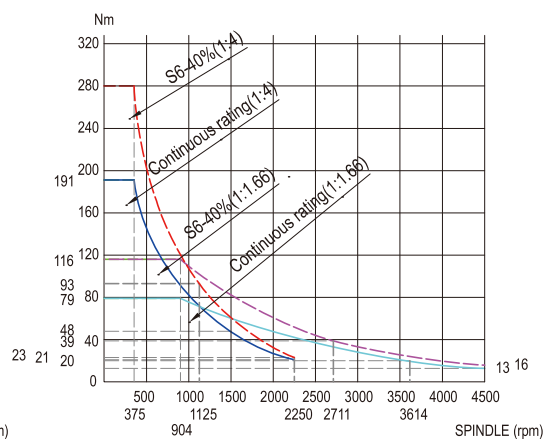
Torque Chart
