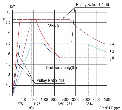
Horsepower Chart
