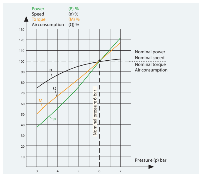
Torque / speed reaction with air regulation
