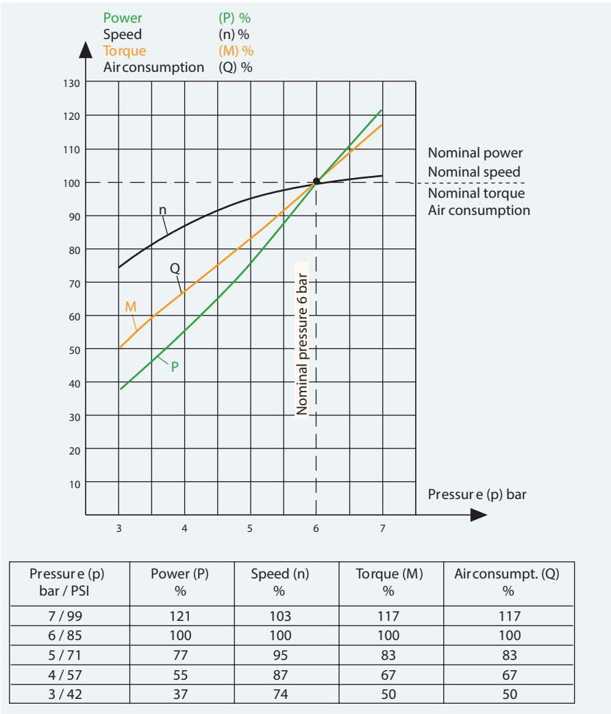
Influences of the operating pressure
