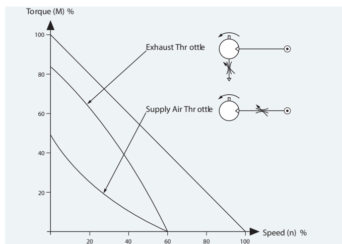
Torque / speed reaction with air regulation
